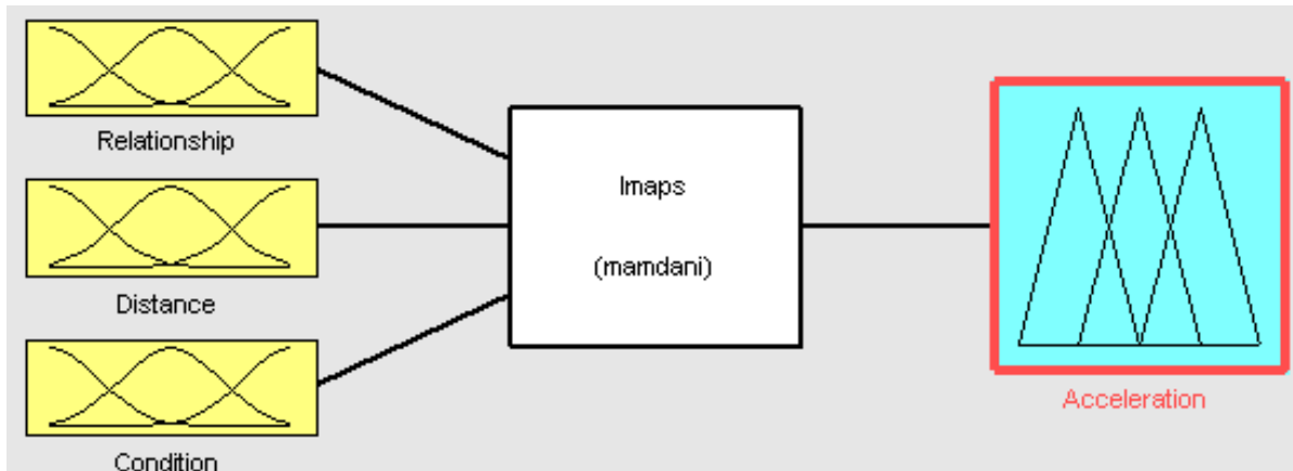
Figure 3. Fuzzy engine
